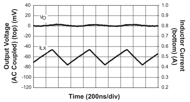
Output Ripple ( V_{IN} = 3.6V ; V_{OUT} = 1.8V ; I_{OUT} = 500mA )
