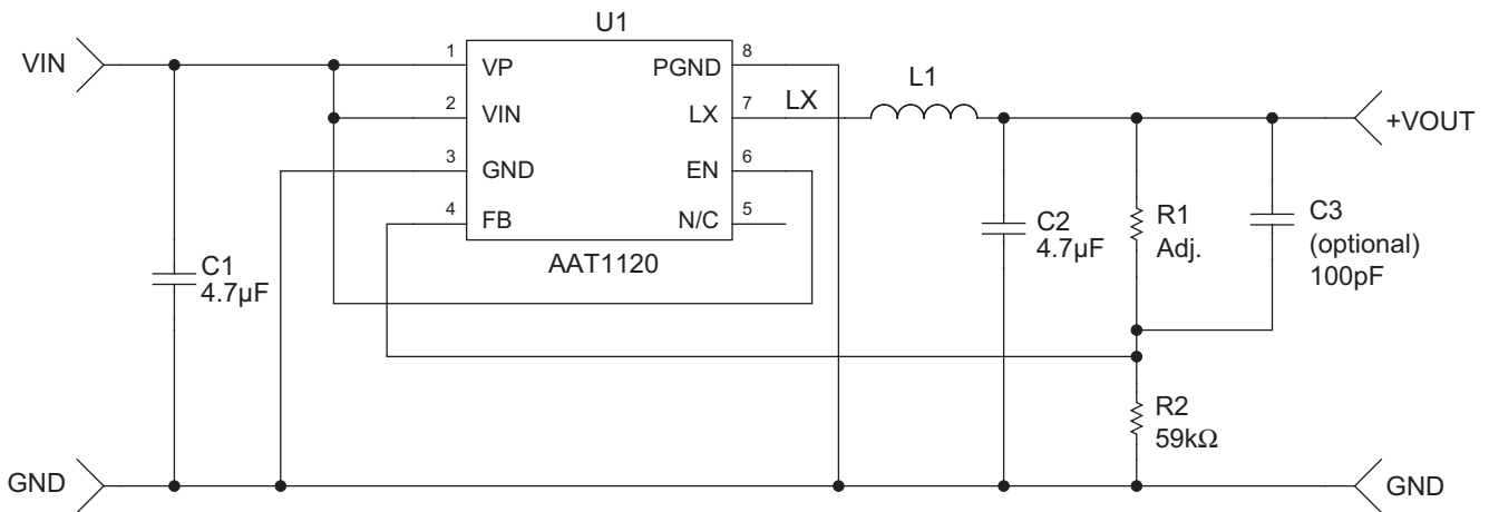
Figure 1: AAT1120 Schematic.
